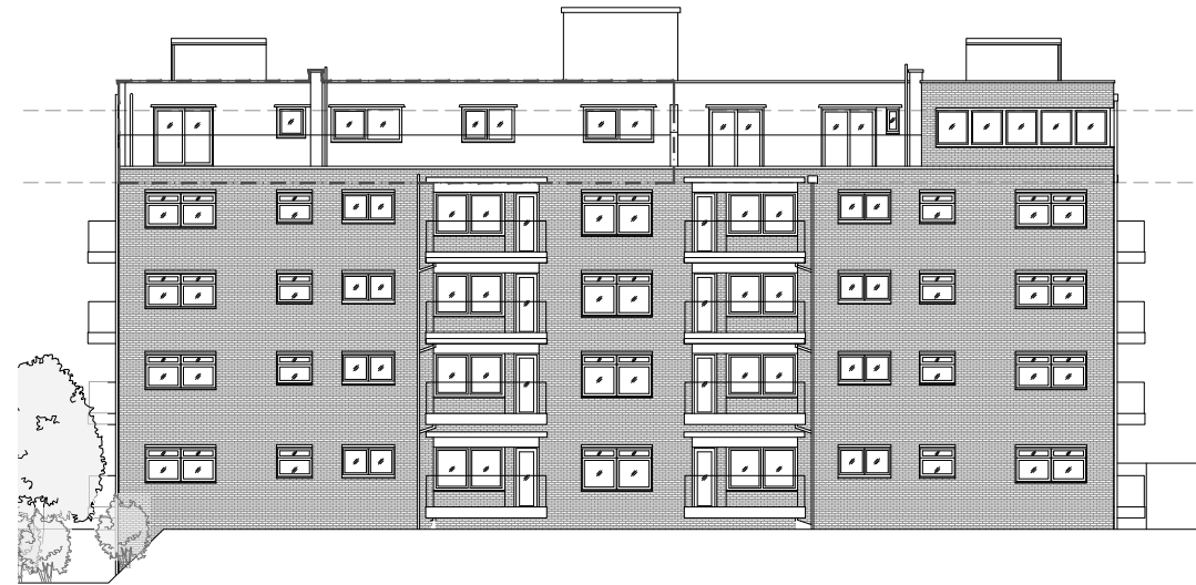
EXISTING APARTMENT REAR (GARDEN) ELEVATION 1:100 @ A1
